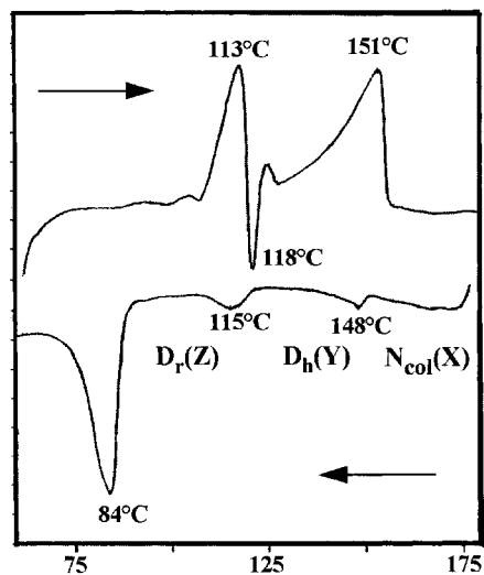
Figure 1. DSC thermogram of the salt 1a (5°C min -1 ): (→) heating, (←) cooling.
