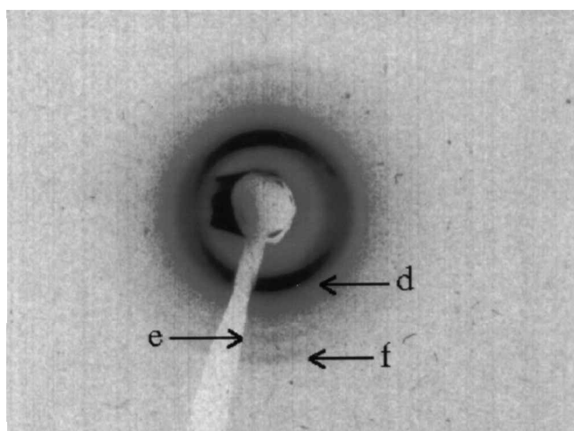
Figure 3. X-ray diffraction pattern of salt 1a in the D_h phase at 140^\circ\text{C} after cooling in the magnetic field (1.7 T). Top: a and b , s=1/38.5 \text{ \AA}^{-1} and s=1/19.3 \text{ \AA}^{-1} , respectively; c , s=1/4.5 \text{ \AA}^{-1} . Bottom: magnification of the small angles region; d , e and f , s=1/38.5 , 1/22.2 and 1/19.3 \text{ \AA}^{-1} , respectively.
